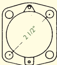
Senior Gauge 2 1/2" Bolt Circle
