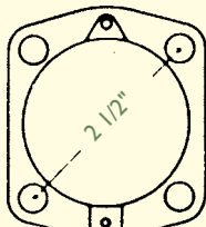
Senior Gauge 2 1/2" Bolt Circle
