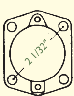
Junior Gauge 2 1/32" Bolt Circle
